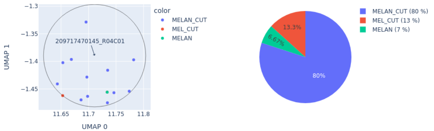
Close-up of UMAP for 209717470145_R04C01 reference: AllIDATv2_20210804_HPAP_Sarc.xlsx (19967 cases), 0 CpGs
