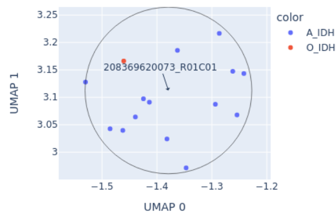
Close-up of UMAP for 208369620073_R01C01 reference: AllIDATv2_20210804_HPAP_Sarc.xlsx (19967 cases), 0 CpGs
