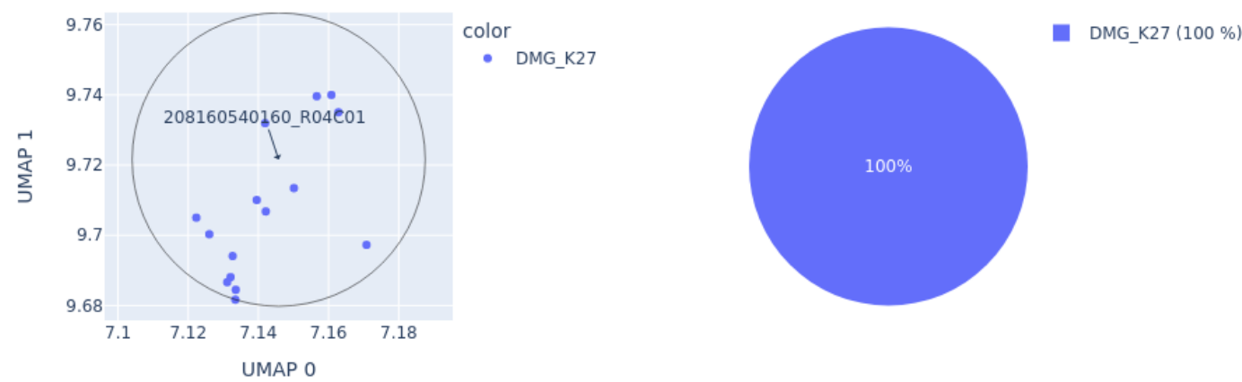
Close-up of UMAP for 208160540160_R04C01 reference: AllIDATv2_20210804_HPAP_Sarc.xlsx (19967 cases), 0 CpGs
