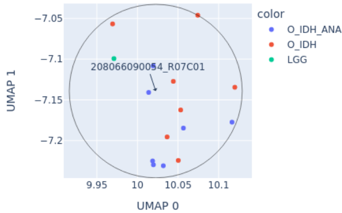
Close-up of UMAP for 208066090054_R07C01 reference: AllIDATv2_20210804_HPAP_Sarc.xlsx (19967 cases), 0 CpGs
