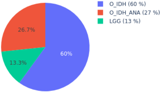
Neighbors in UMAP for 206486310053_R07C01 reference: AllIDATv2_20210804_HPAP_Sarc.xlsx (19967 cases), 0 CpGs
