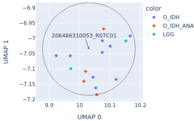
Close-up of UMAP for 206486310053_R07C01 reference: AllIDATv2_20210804_HPAP_Sarc.xlsx (19967 cases), 0 CpGs
