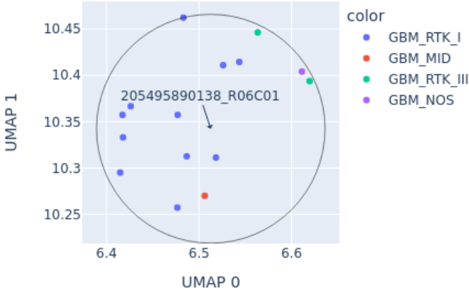
Close-up of UMAP for 205495890138_R06C01 reference: AllIDATv2_20210804_HPAP_Sarc.xlsx (19967 cases), 0 CpGs
